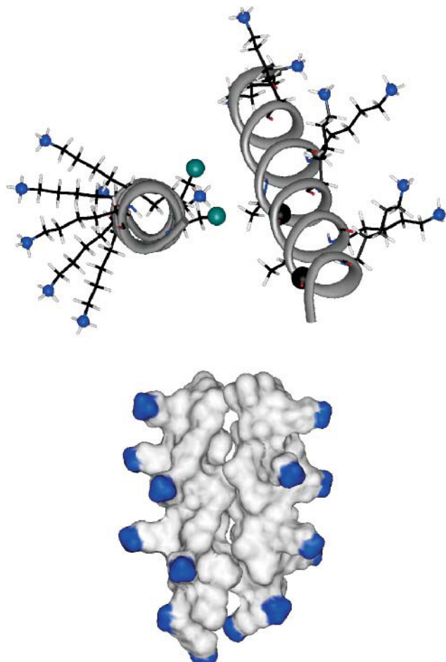
FIGURE 10 (Top) Side groups of the K3 dimer. Only the labeled residues ( \text{Ala}_{10} and \text{Ala}_{17} of one chain, and \text{Ala}_{10} and \text{Ala}_{14} of the other) as well as the lysine side chains are shown. The ^{13}\text{C} and ^{19}\text{F} labels are shown as black and green balls, respectively, and the amino nitrogens as blue balls. The approximate tilt angle of the two helices is 20^\circ . (Bottom) Surface representation of the K3 dimer. The amino-terminus of the peptide and the terminal amino groups of the protruding lysine side chains are blue.
