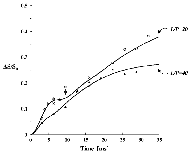
FIGURE 3 50.3-MHz ^{13}\text{C}\{^{19}\text{F}\} REDOR dephasing ( \Delta S/S_0 ) for a 50-50 mixture of [1\text{-}^{13}\text{C}]\text{Ala}_{10}\text{-}[^{15}\text{N}]\text{Gly}_{11}\text{-(KIAGKIA)}_3\text{-NH}_2 and [2\text{-}^2\text{H}, 3\text{-}^{19}\text{F}]\text{Ala}_{10}\text{-(KIAGKIA)}_3\text{-NH}_2 , incorporated into synthetic MLVs of DPPG/DPPC (1:1) at a lipid/peptide molar ratio of 20 (○) and 40 (▲). Root mean-square deviation errors are indicated by the vertical lines for the first six evolution times ( L/P = 20 ). Both samples were lyophilized in a protecting sugar matrix. The crosses show dephasing for the frozen fully hydrated ( L/P = 20 ) sample of Fig. 2 (top). The solid lines show the calculated dephasing assuming two distributions of ^{13}\text{C}\text{-}^{19}\text{F} pair distances. At L/P = 20 , the two distributions are about equally populated and the difference in average dephasing rates for the two populations is more than a factor of two. Based on signal/noise ratios, the root mean-square deviation uncertainty in the dephasing ( \Delta S/S_0 ) is estimated at 5% (see footnote to Table 1). One distribution has a mean internuclear ^{13}\text{C}\text{-}^{19}\text{F} separation of 4.5 Å with a width of 0.7 Å, and the other distribution has a mean of 9.6 Å and a width of 3.0 Å. At L/P = 40 , the population with the smaller mean and narrower distribution width decreases.
