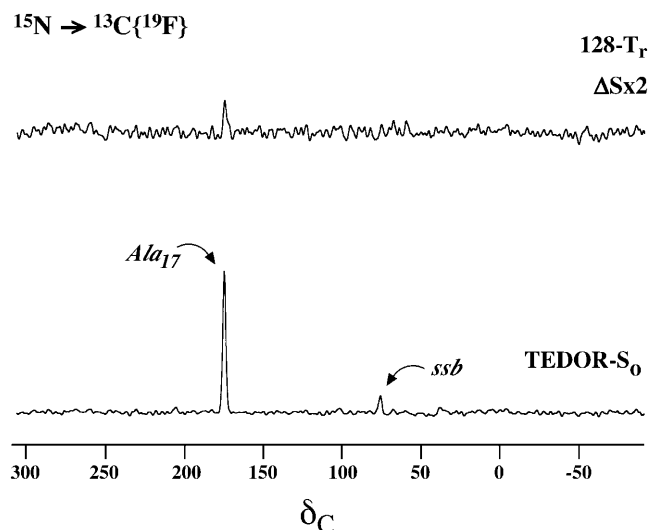
FIGURE 5 50.3-MHz ^{15}\text{N} \rightarrow ^{13}\text{C}\{^{19}\text{F}\} TEDOR-REDOR NMR spectra of a 50-50 mixture of ([3-^{13}\text{C}]\text{Ala}_3-[^{15}\text{N}]\text{Gly}_4-[^{13}\text{C}]\text{Ala}_{10}-[2-^{13}\text{C}]\text{Gly}_{11}-[6-^{15}\text{N}]\text{Lys}_{12}-[1-^{13}\text{C}]\text{Ala}_{17}-[^{15}\text{N}]\text{Gly}_{18}) -NH _2 and [2-^2\text{H}, 3-^{19}\text{F}]\text{Ala}_{14} -(KIAGKIA) _3 -NH _2 , incorporated into synthetic MLVs of DPPG/DPPC (1:1) at a lipid/peptide molar ratio of 20 after 128 rotor cycles of dipolar evolution with magic-angle spinning at 5000 Hz. The spectrum at the bottom resulted from a 4- T_r , ^{15}\text{N} \rightarrow ^{13}\text{C} TEDOR coherence transfer followed by 128 additional rotor cycles with high power proton decoupling. The 128- T_r REDOR \Delta S spectrum of the TEDOR-selected signal is shown at the top of the figure.
