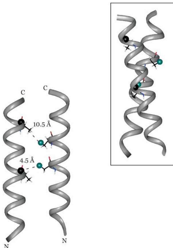
FIGURE 9 Model of the dimerized K3 chains obtained from the combination of distance and angular information. After energy minimization, the [1\text{-}^{13}\text{C}]\text{Ala}_{10}\text{-}[3\text{-}^{19}\text{F}]\text{Ala}_{10} and the [1\text{-}^{13}\text{C}]\text{Ala}_{17}\text{-}[3\text{-}^{19}\text{F}]\text{Ala}_{14} interchain distances are 4.5 Å and 10.5 Å, respectively. The REDOR determined distances are 4.5 Å and 10.4 Å. The helices intersect at an approximate cross-angle of 20^\circ (inset).
