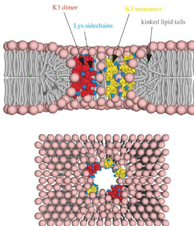
FIGURE 13 Cartoons of the pore model: cross section ( top ) and top view ( bottom ). (KIAGKIA) 3 -NH 2 monomers and dimers are shown in yellow and red, respectively. The lysine side chains are indicated by blue. Peptide chains and lipid headgroups together line the wall of the torus-like pore. A few of the kinked lipid chains have ^{19}\text{F} -labeled tails (in green ) near the phospholipid headgroups.
